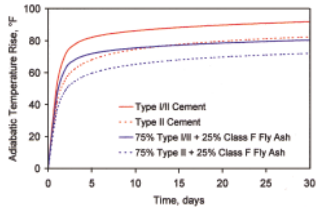
Fig. 3: Concrete temperatures of mixes with 525 lb/yd 3 of cementitious materials
