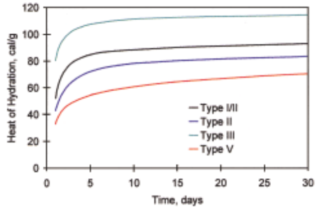
Fig. 2: Heat of hydration for typical cements
